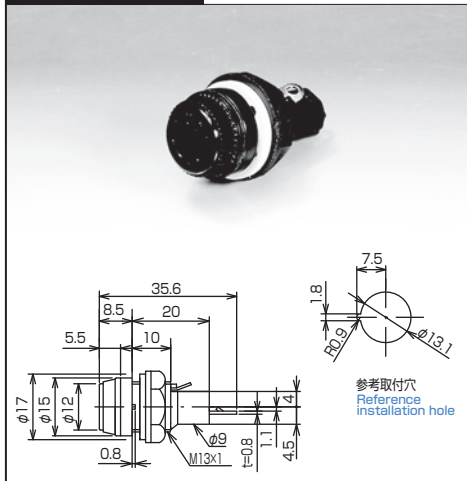
FH-B02 Fuse Holder
