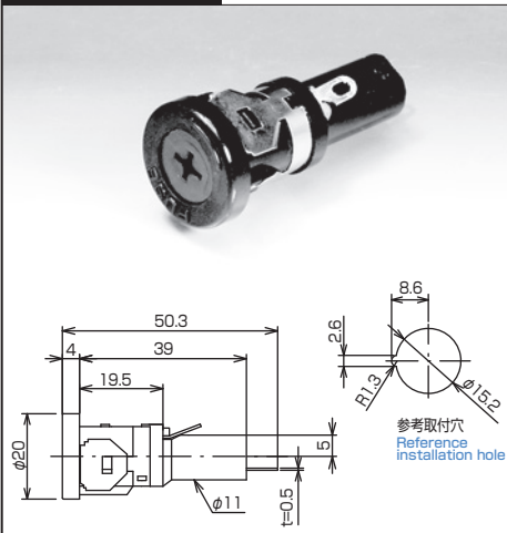
FH-S07 Fuse Holder
