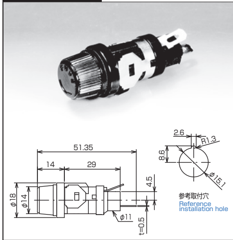
FH-043A Fuse Holder
